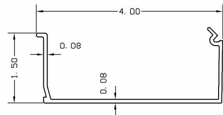
5- PHX-504 INSULATED GLASS STOP
