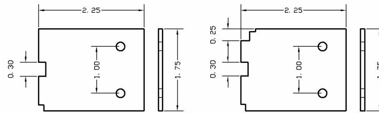
10- 0.09" x 2.25" x 1.75" ALUMINUM MALE END CAP
