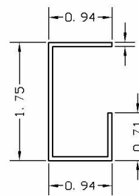
23- #1 JAMB CLOSURE
